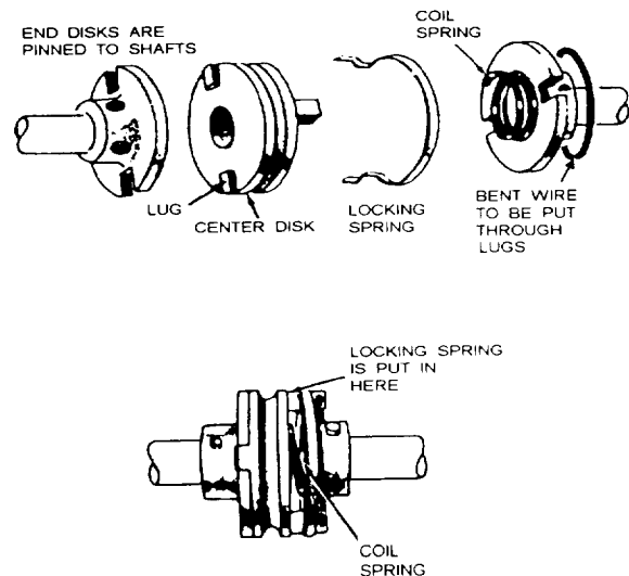
Figure 11-16.-Oldham coupling.
