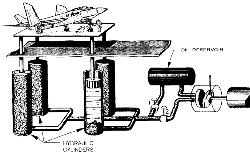
Figure 10-12.-Hydraulic lift.
